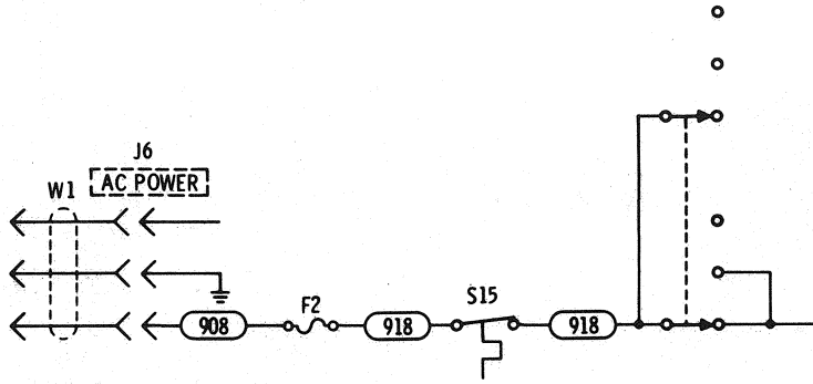
Figure 6. Partial Schematic Diagram of the Power Supply Section Showing Thermal Switch S15 (Part of Change 10)
